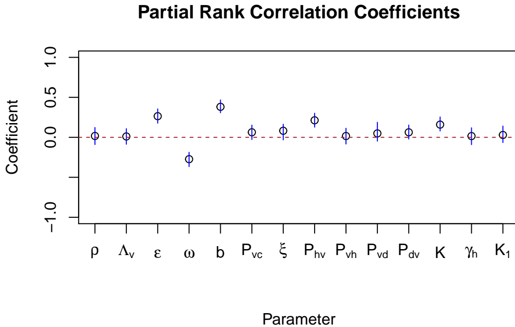
Figure 36 – Partial Rank Correlation Coefficients for the 14 parameters dimension for different q values.
