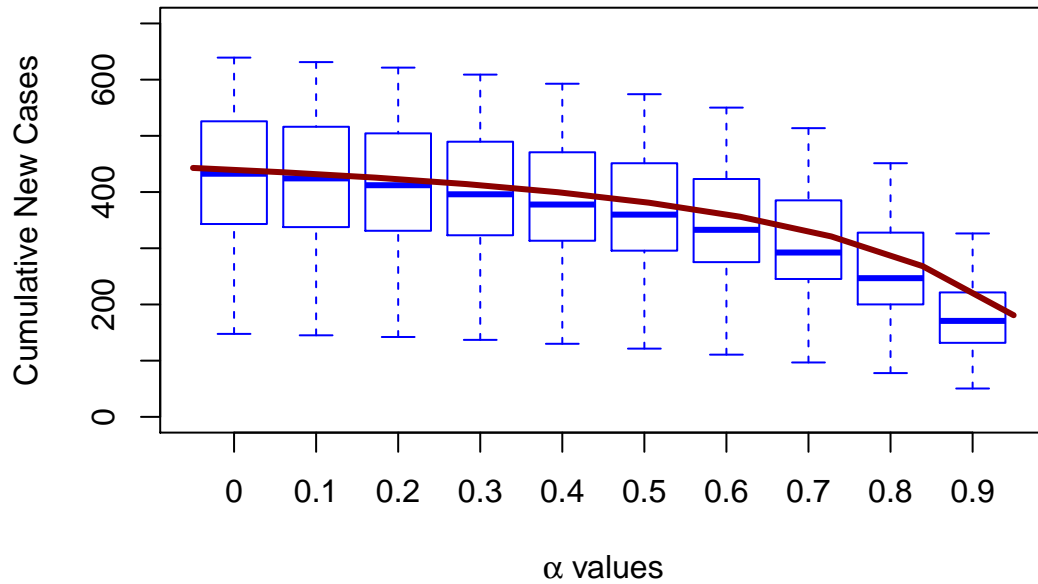
Figure 33 – Cumulative number of new cases for different effectiveness on house improvement and hygiene, represented by the parameter \alpha . For each value of \alpha , 100 simulations of the model were performed using Latin Hypercube Sampling for uncertain parameters. The red line represents the average behavior of the cumulative number of new cases when the parameters assume their baseline values.
