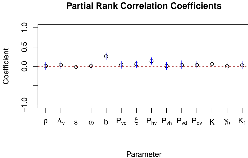
Figure 38 – Partial Rank Correlation Coefficients for the 14 parameters for different values of \delta_{ins} .
