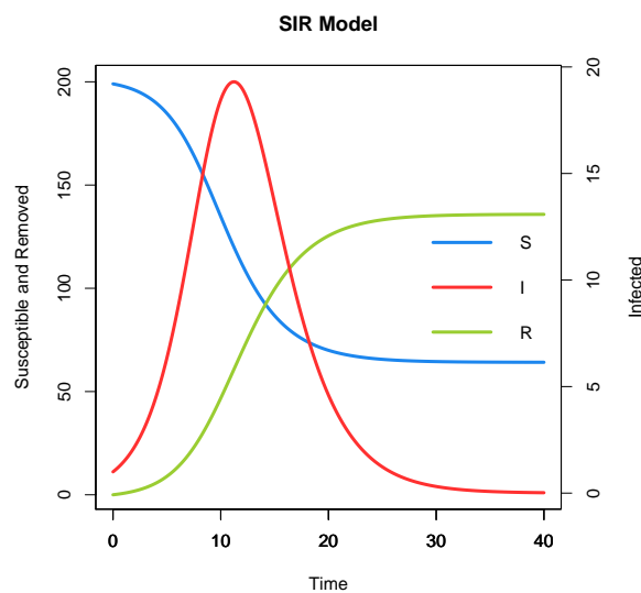
Figure 9 – Plot showing the dynamics for the SIR (susceptible-infected-recovered) model.
