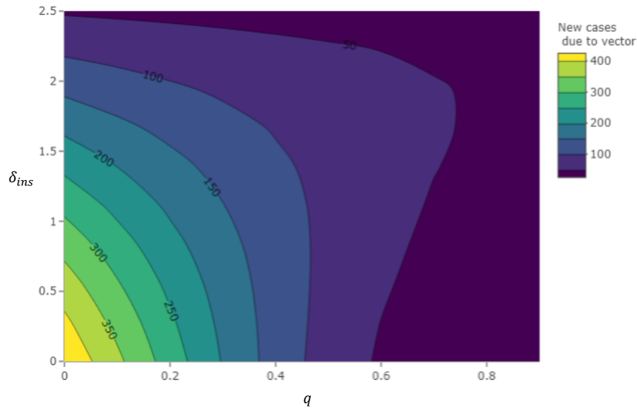
Figure 31 – Contour plot showing the effects caused by combination of spraying insecticides and usage of door and windows screen on the number of new cases due to vector.
