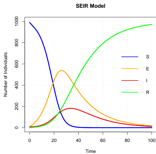
Figure 11 – Plot for SEIR model.
