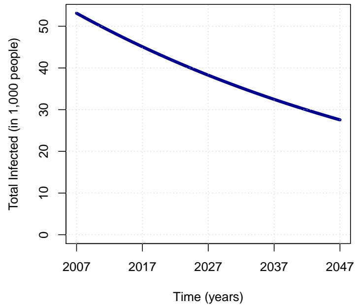
Figure 15 – Dynamics on the number of total infected people along 40 years simulation considering death rate due to disease as twice the natural death rate and no migration flows.
