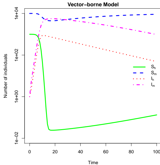
Figure 13 – Graph showing the vector-borne dynamics for susceptible and infected human and mosquitoes.
