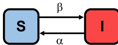
Figure 6 – Flow chart for a SIS (susceptible-infected-susceptible) model.
