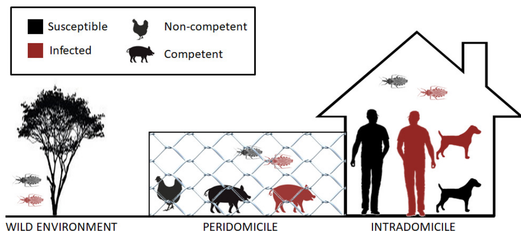
Figure 22 – Illustrative representation of the elements considered in the compartmental model: human, vector, competent and non-competent hosts. All of them can be found in a susceptible or infected epidemiological state. Also two environments were considered, the peridomicile and the intradomicile.
