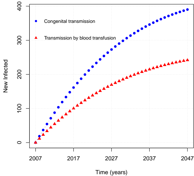
Figure 16 – Comparison of the number of cumulative new infections along time when a single transmission route is considered.
