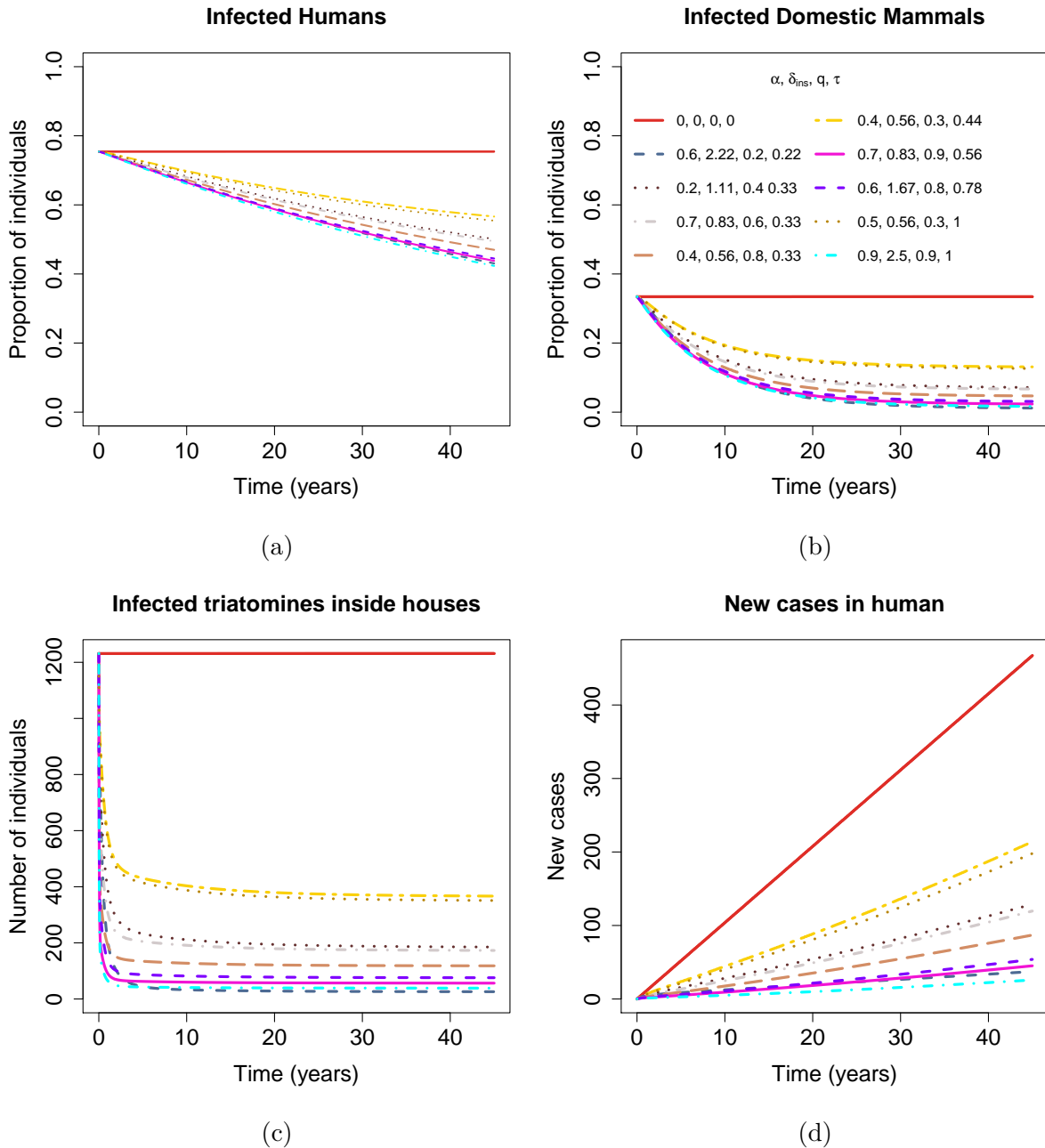
Figure 28 – Effect of combined control strategies: house improvement and hygiene, usage of windows and door screen, and spraying residual insecticides. Figures show (a) the proportion between infected humans and total human population, (b) the proportion between infected domestic mammals and total population of domestic mammals, (c) the number of infected vectors inside house, and (d) the cumulative number of new cases in human due to vector transmission, for different parameters combination.
