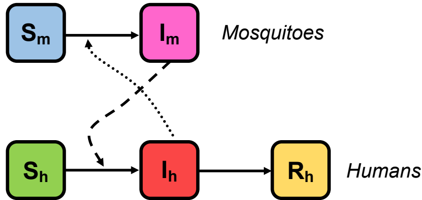
Figure 12 – A flow chart representing a vector-borne dynamics where the compartments are: S_h : susceptible human, I_h : infected human, R_h : recovered human, S_m : susceptible mosquitoes and I_m : infected mosquitoes.
