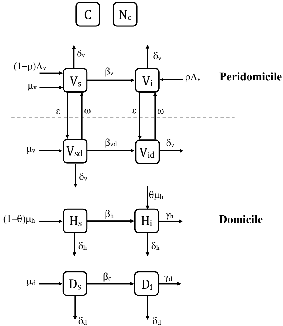
Figure 23 – Flow chart representing the compartmental model for a community. C represents the competent hosts in peridomicile and N_c the non-competent hosts. Both are considered constant, that is why there is no arrow associated with them. V_s and V_i are susceptible and infected vectors in the peridomicile, respectively. V_{sd} and V_{id} represent susceptible and infected vectors inside house, respectively. H_s represents susceptible humans, and H_i infected ones. D_s and D_i represents susceptible and infected domestic mammals respectively. Arrows indicate the flows on the compartments. \mu represents birth rates, \delta represents mortality rates, \gamma represents mortality rate due to the disease, \beta represents the force of infection.
