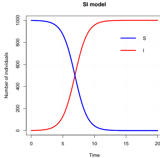
Figure 5 – SI model (Susceptible - Infected) dynamics over time.
