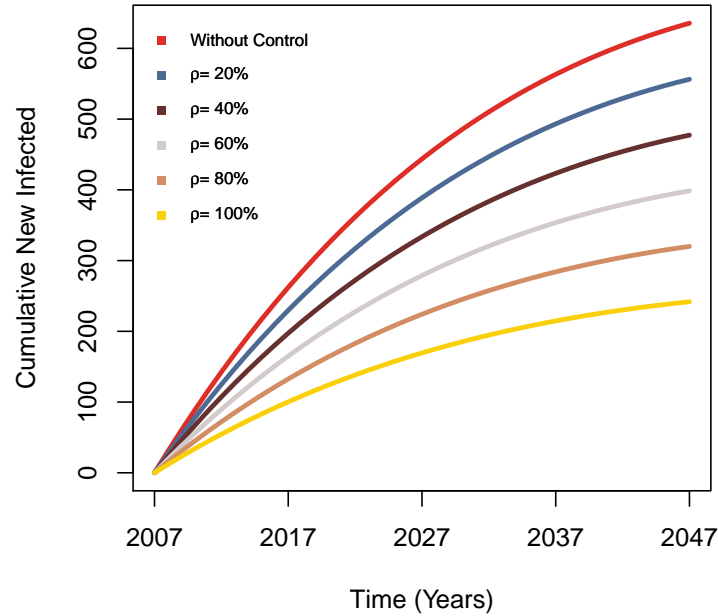
Figure 17 – Sensitivity analysis on the cumulative number of newly infected individuals by varying \rho , i.e., the proportion of treatment of infected newborn.
