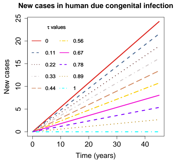
Figure 27 – Effect of treatment of women in childbearing age on the number of new congenital cases. The parameter associated with treatment is \tau and, it is in the range 0 \leq \tau \leq 1 . \tau = 0 represents the scenario without control and, \tau = 1 represents a totally effective control strategy.
