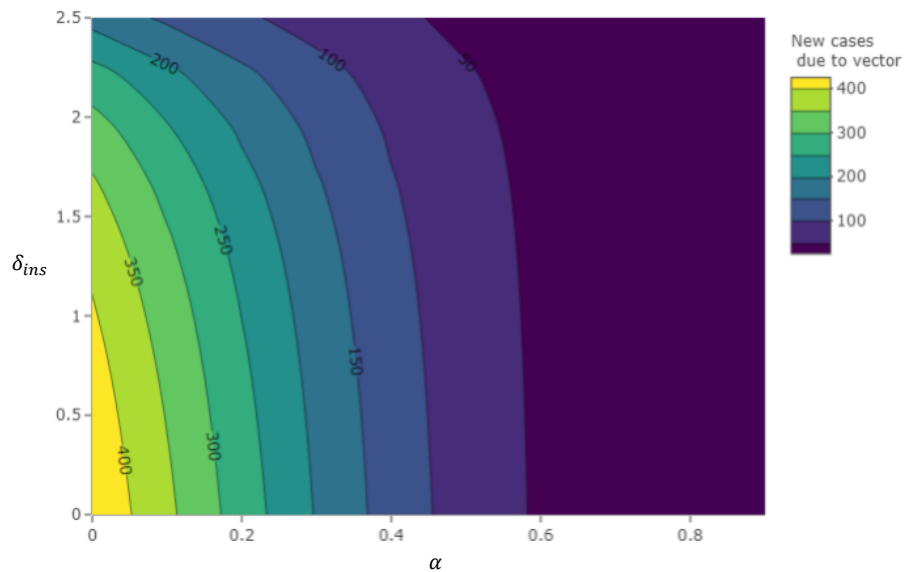
Figure 30 – Contour plot showing the effects caused by combination of house improvement and hygiene, and spraying insecticides on the number of new cases due to vector.
