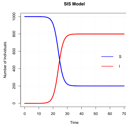
Figure 7 – SIS (susceptible-infected-susceptible) model dynamics over year.
