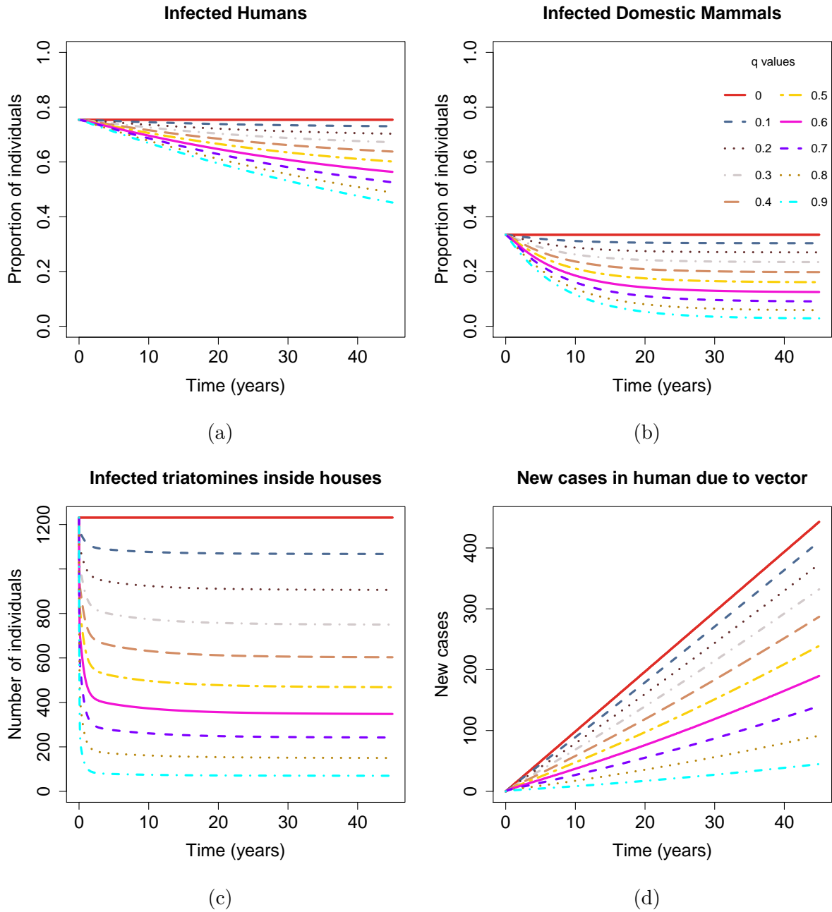
Figure 26 – Effects produced by usage of door and window screen. This control strategy is modeled by varying the vector movement rate from peridomicile to intradomicile by a factor q , representing the effectiveness of this control strategy. The range used was 0 \leq q \leq 1 . Figures show (a) the proportion between infected humans and total human population, (b) the proportion between infected domestic mammals and total population of domestic mammals, (c) the number of infected vectors inside house, and (d) the cumulative number of new cases in human due to vector transmission, for different q values.
