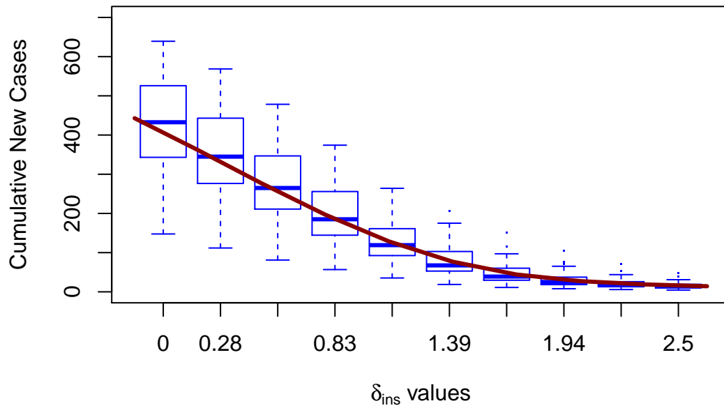
Figure 37 – Cumulative number of new cases for different
