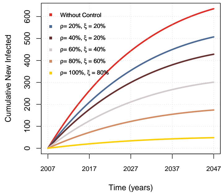
Figure 19 – Sensitivity analysis on the cumulative number of newly infected by applying combined control – increasing proportion of treatment in infected newborns (parameter \rho ) and on the surveillance in blood transfusion transmission (parameter \xi ).
