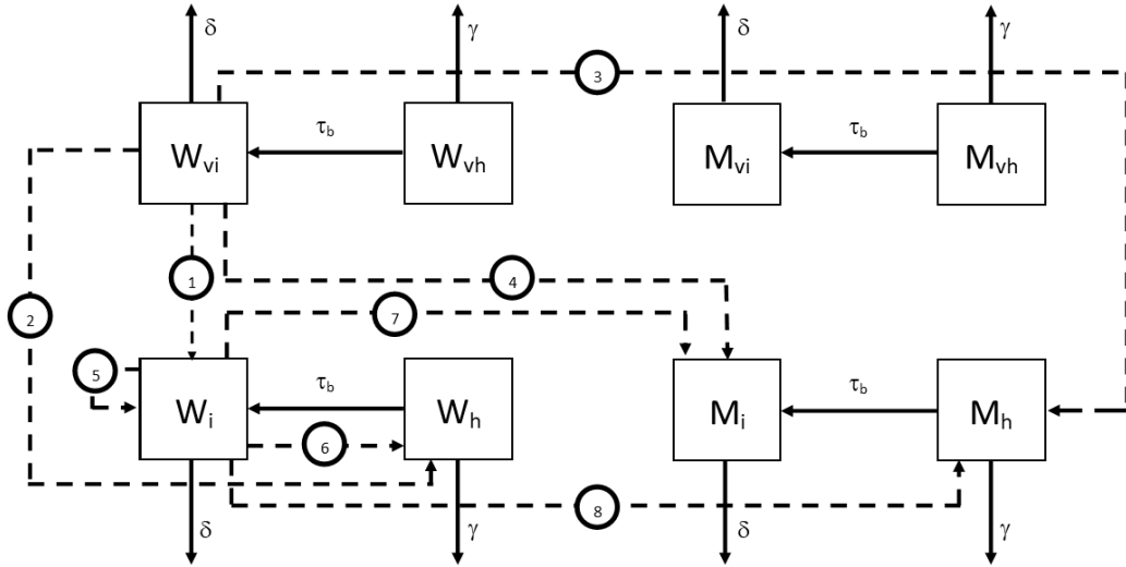
Figure 14 – Flow chart for the dynamics of the proposed model. Letters inside box indicate the number of individuals in each compartment: infected women from country with vector ( W_{vi} ), healthy women from country with active vector transmission ( W_{vh} ), infected men from country with active vector transmission ( M_{vi} ), healthy men from country with active vector transmission ( M_{vh} ), infected women from country without vector transmission ( W_i ), healthy women from country without vector transmission ( W_h ), infected men from country without vector transmission ( M_i ), healthy men from country without vector transmission ( M_h ). \gamma is the death rate for healthy people and \delta is the death rate for infected people. \tau_b is the rate of infection due to blood transfusion. Dashed lines indicate births. Newborns from W_{vi} can be an infected female (1), healthy female (2), healthy male (3) or infected male (4). The same occurs for newborns from W_i that can be infected female (5), healthy female (6), infected male (7) or healthy male (8). Healthy women W_{vh} and W_h only gave birth to healthy newborns (flows not shown).
