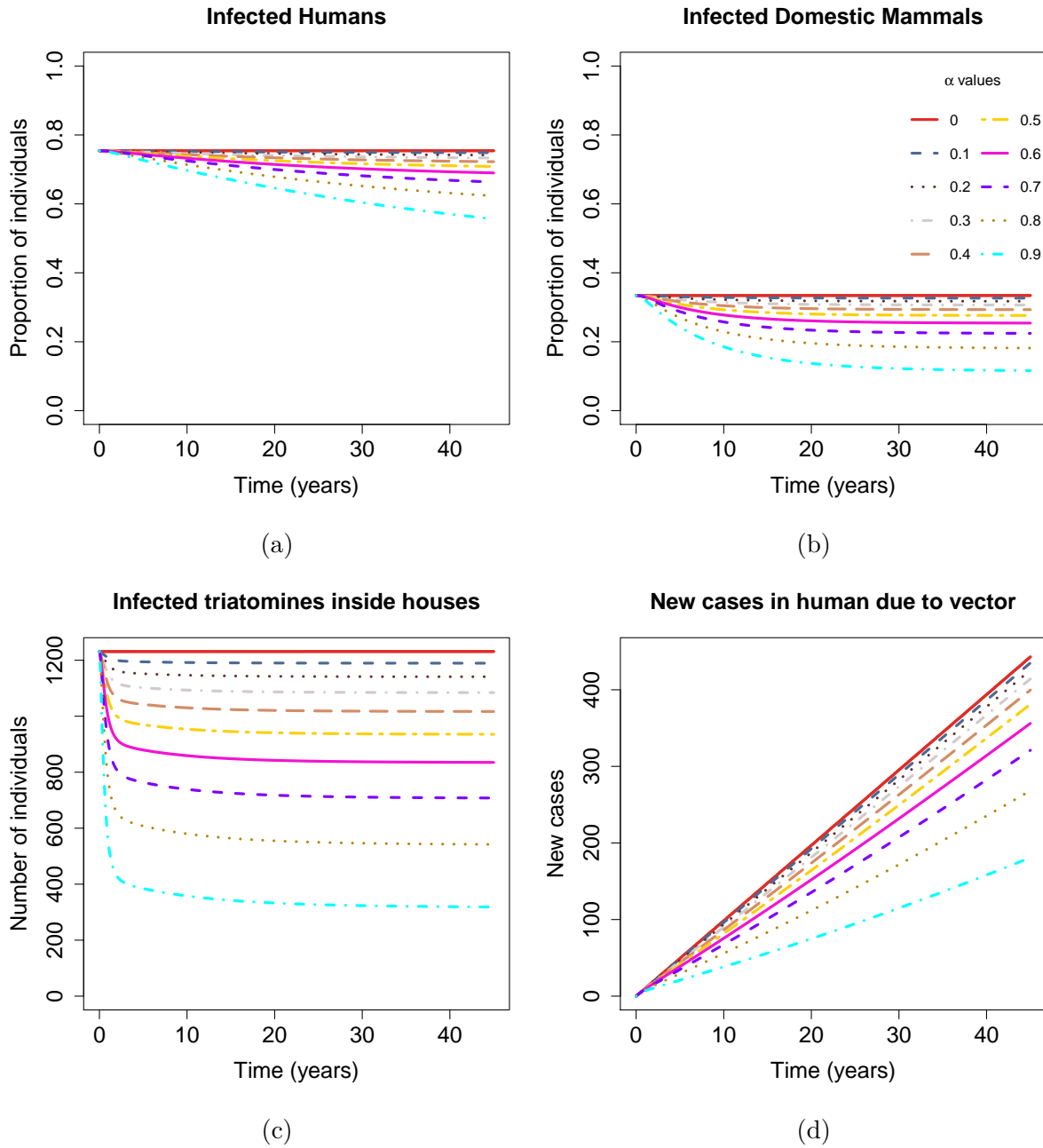
Figure 24 – Effects produced by house improvement and hygiene, represented by the parameter \alpha ; in (a) the proportion of infected humans; in (b) the proportion of infected domestic mammals; in (c) the number of infected vectors inside the house; in (d) the cumulative number of new cases in human due to vector infection. \alpha ranges from 0 to 0.9.
