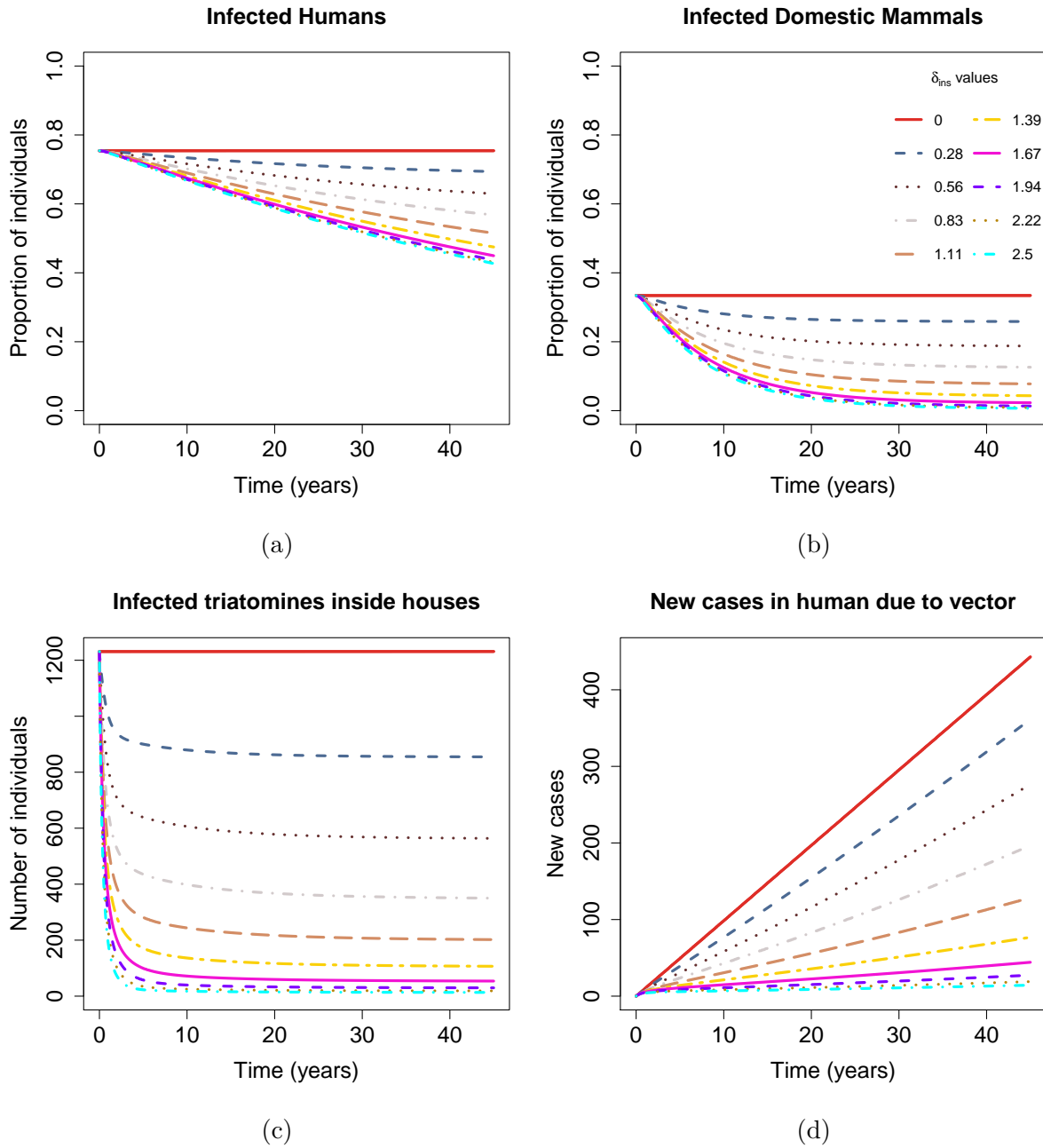
Figure 25 – Effects produced by spraying residual insecticide. Figures show (a) the proportion between infected humans and its population, (b) the proportion between infected domestic mammals and its total population, (c) the number of infected vectors inside the house, and (d) the cumulative number of new cases in human due to vector infection. \delta_{ins} , vary from 0 to 2.5 times the natural mortality rate for vectors ( \delta_v ).
