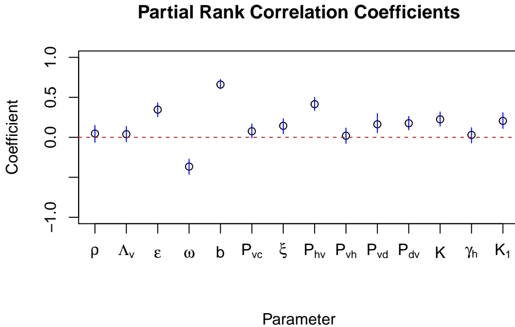
Figure 34 – Partial Rank Correlation Coefficients for the 14 parameters dimension.
