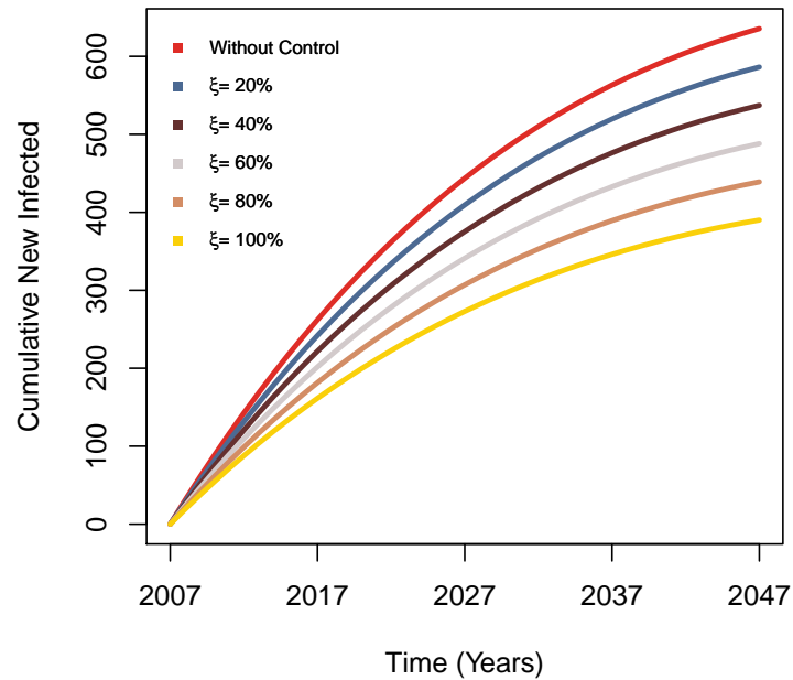
Figure 18 – Sensitivity analysis on the cumulative number of newly infected individuals by varying \xi , i.e., the probability of effective surveillance in blood transfusions.
