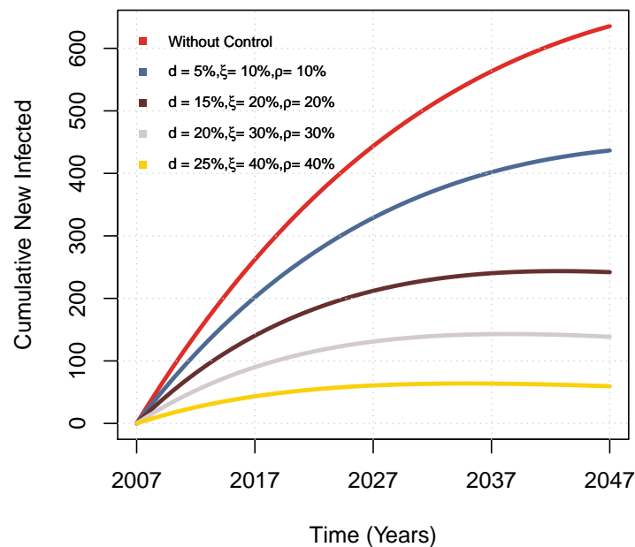
Figure 20 – Sensitivity analysis considering detection and treatment of infected individuals d , treatment of infected newborns \rho and surveillance in blood transfusion transmission \xi .
