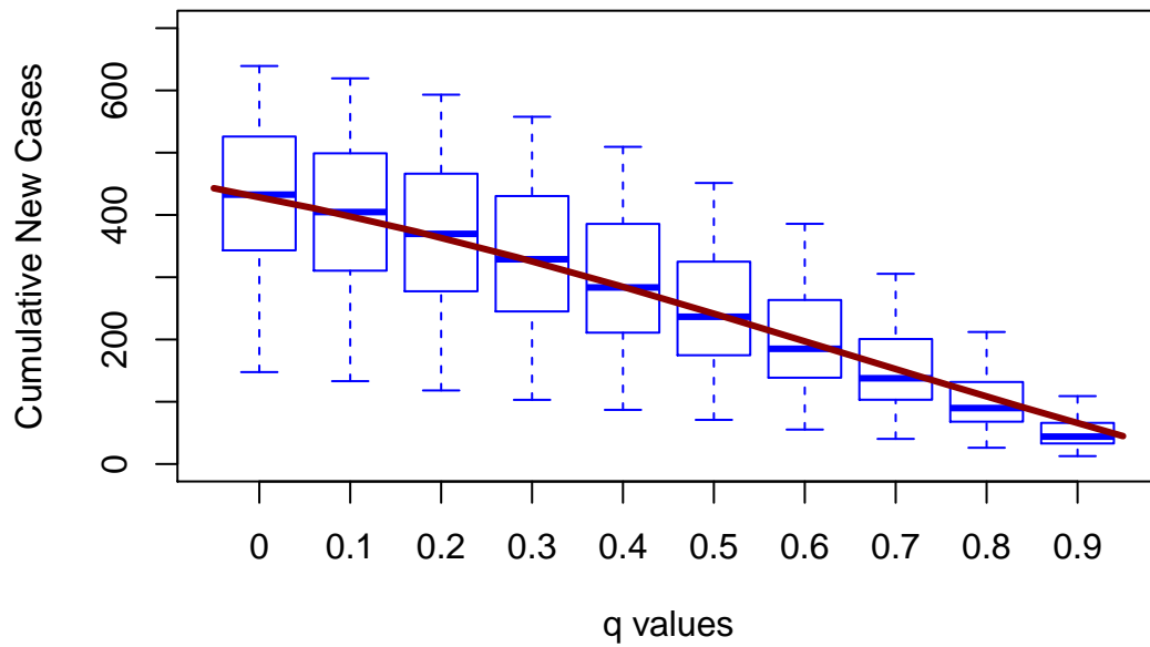
Figure 35 – Cumulative number of new cases for different effectiveness on the usage of door and window screen, represented by the parameter q . For each value of q , 100 simulations of the model were performed. For each simulation the parameters were generated using Latin Hypercube Sampling.
