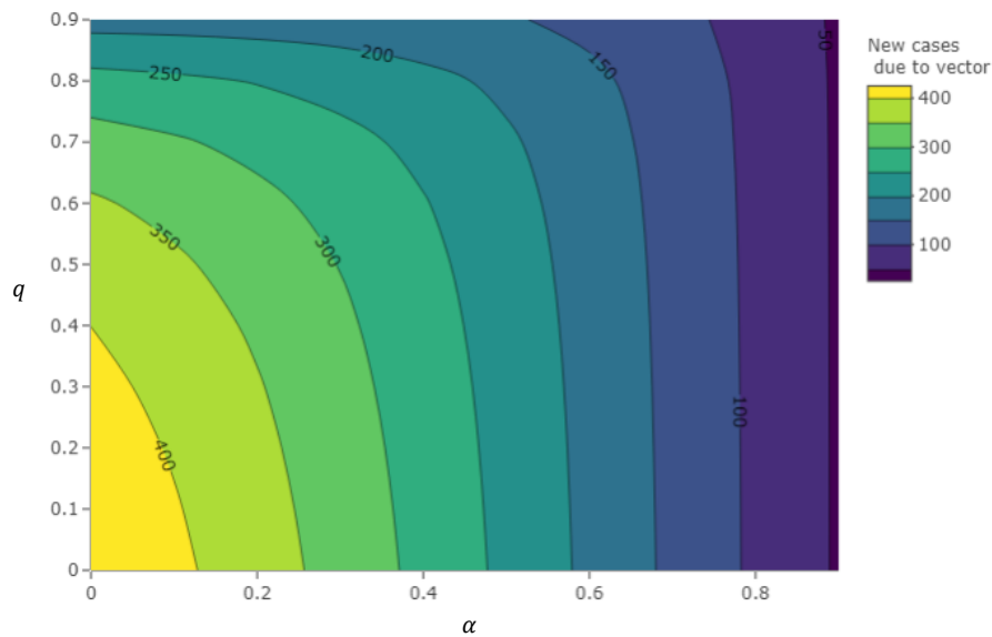
Figure 29 – Contour plot showing the effects caused by combination of house improvement and hygiene, and usage of door and windows screen on the number of new cases due to vector.
