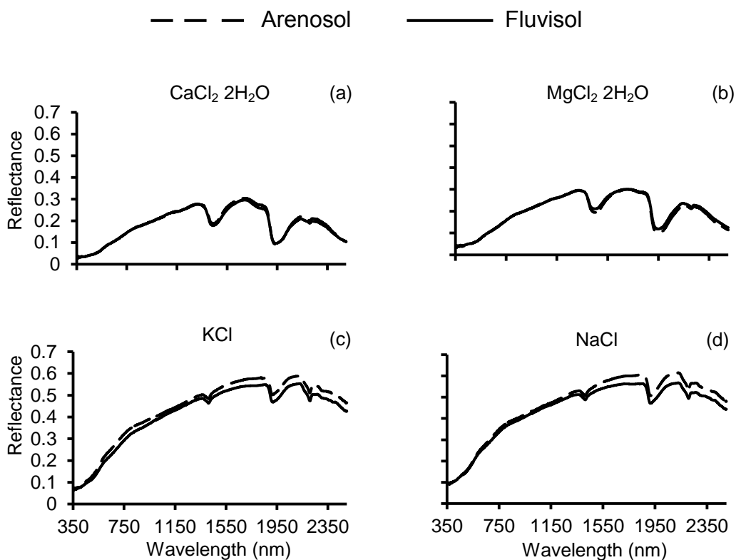
Figure 2.4. Spectral signatures of soils for salts of \text{CaCl}_2 \cdot 2\text{H}_2\text{O} , \text{MgCl}_2 \cdot 2\text{H}_2\text{O} , KCl and NaCl.
