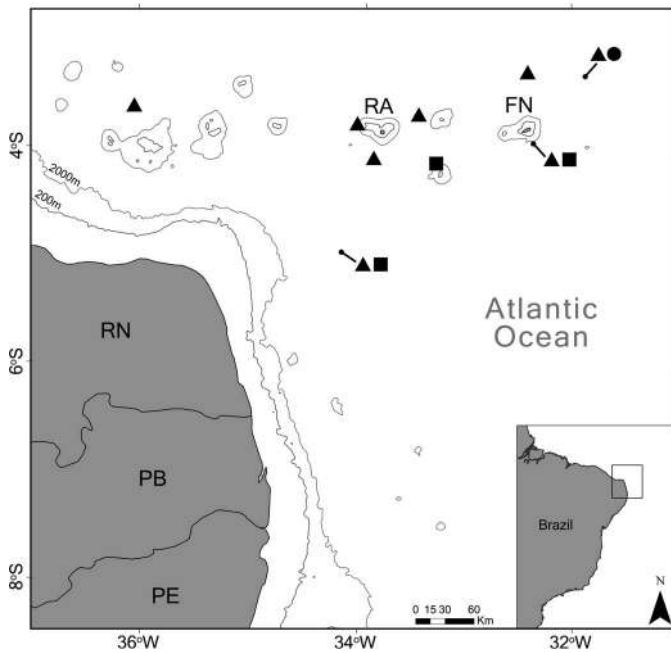
Fig. 4. Records of Scopeloberyx opercularis (circle), Scopeloberyx opisthopterus (square), and Scopelogadus mizolepis (triangle) off northeastern Brazil collected during the ABRACOS surveys. Tip of arrow indicates same collection locality for different species. FN—Fernando de Noronha Archipelago; PB—Paraíba; PE—Pernambuco; RA—Rocas Atoll; RN—Rio Grande do Norte.
