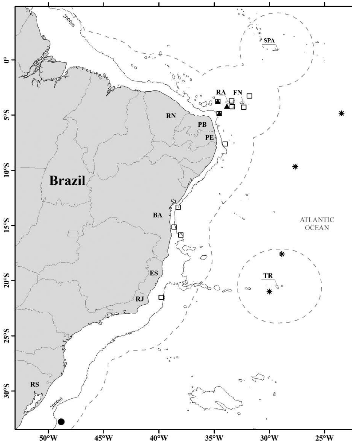
Figure 2. Distribution of Bathysphyaenops simplex (full triangle) and Howella atlantica (open square) examined in the present study. Previous records of Howella atlantica (asterisk) and Howella sherborni (full circle) along Brazilian waters (from Post and Quéro 1991). Limits of the Brazilian Exclusive Economic Zone in dash line. Oceanic islands: SPA – São Pedro e São Paulo Archipelago; RA – Rocas Atoll; FN – Fernando de Noronha Archipelago; TR – Trindade Island. Selected Brazilian states: RN – Rio Grande do Norte; PB – Paraíba; PE – Pernambuco; BA – Bahia; ES – Espírito Santo; RJ – Rio de Janeiro, RS – Rio Grande do Sul.
