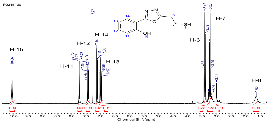
Figura 12. Espectro de RMN ^1\text{H} (300 MHz, \text{CDCl}_3 ) do 1,3,4-oxadiazol.
